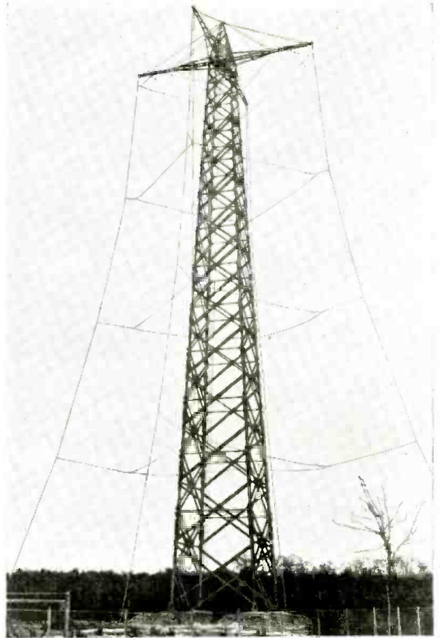
Above—The "round-radiation" antenna, "rundstrahler", used for vertical concentration of the radiated waves. Left—Aerial view of transmitting station at Zeesen, showing the masts supporting the directional antennas and also the building housing the transmitting equipment.
