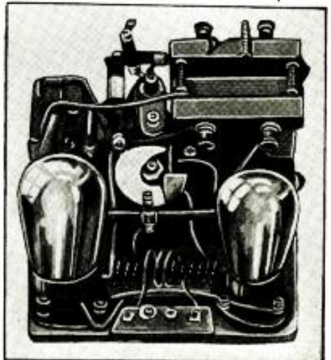
Behind the panel view, showing how the various parts of the 5-meter "Transceiver" are mounted.
