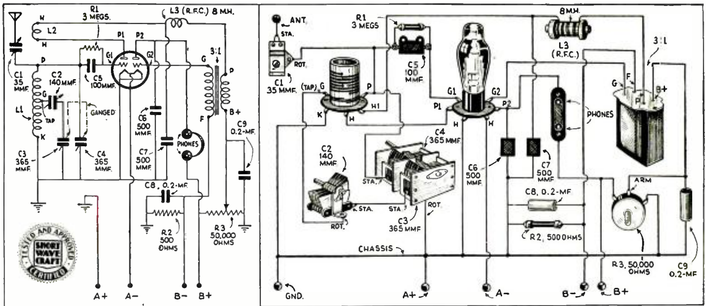
Practically anyone, even though they are not familiar with the construction of radio sets, can by carefully following the diagrams above, successfully build the "Constant Band-Spread" Twinplex Receiver. This receiver combines so many desirable features that you will surely want to try it.
