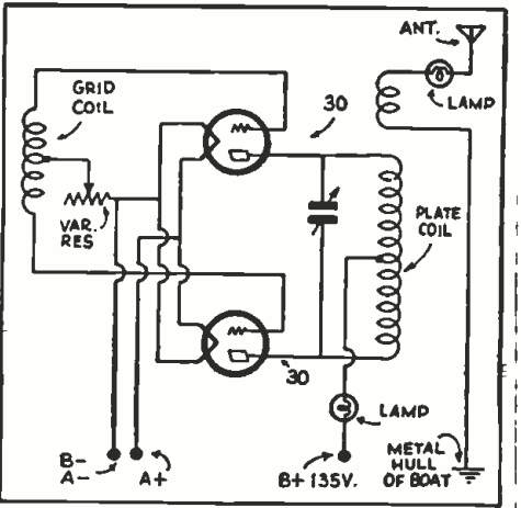
The emergency transmitter hook-up.
