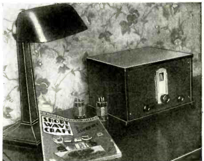
Here is the dandy job which Harry Shepherd made of the "Victor 2-Tube Superhet" receiver, described in our December issue.
