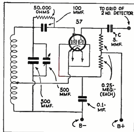
Diagram showing beat-oscillator to be used with any superheterodyne.
